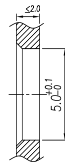
Panel cut-out
